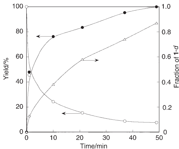
Fig. 1. Reaction of 1 (0.007 mol dm -3 ) in CDCl 3 /HFP- O-d (10/1 v/v) containing sodium alkoxide (0.02 mol dm -3 ) at 297 K, monitored by 1 H NMR: 1 + 1-d (○), PhI (●), and 1-d /( 1 + 1-d ) (△).
